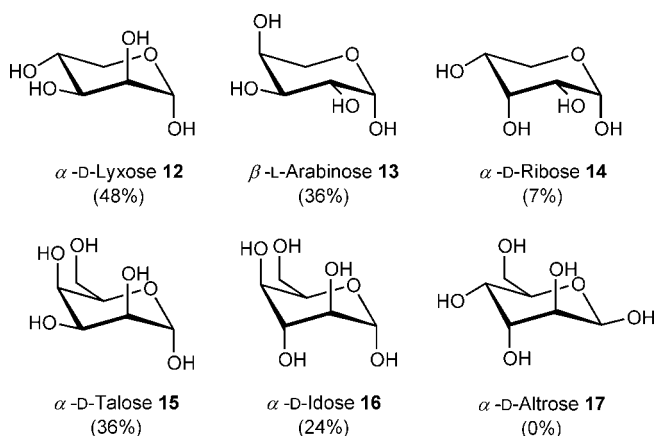
Figure 2. Aldoses as acceptor substrates for recombinant SuSy1 from potato. The monosaccharides (10 mM) were tested with the donor UDP-Glc (2 mM) in 50 mM HEPES buffer, pH 8.0, for 16 h at 30 °C. The formation of disaccharides and the conversion of UDP-Glc was monitored by HPLC. The relative yields refer to the donor substrate UDP-Glc.
