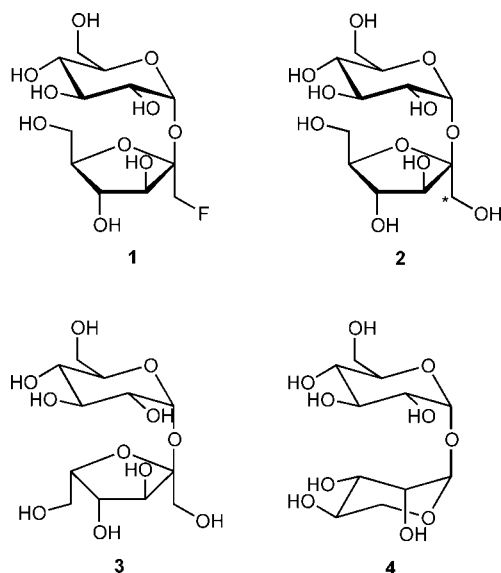
Figure 4. Products of the enzymatic synthesis with recombinant SuSy1: 1-deoxy-1-fluorofructofuranosyl- \alpha -D-glucopyranoside ( 1 ), [ ^{13}\text{C}_1 ]- \beta -D-fructofuranosyl- \alpha -D-glucopyranoside ( 2 ), \alpha -D-glucopyranosyl- \alpha -L-sorbofuranoside ( 3 ), and \alpha -D-glucopyranosyl- \alpha -D-lyxopyranoside ( 4 ).
