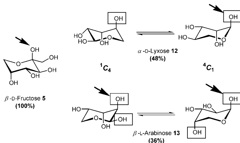
Figure 3. Hypothetical model to demonstrate the isosteric configurations of the hydroxy groups of \alpha -D-lyxose and \beta -L-arabinose in comparison to the {}^1C_4 chair conformation of \beta -D-fructose. Isosteric hydroxy groups are highlighted. Putative sites for the transfer of the donor substrate are indicated by arrows. For \alpha -D-lyxose the model product was confirmed by preparative synthesis and characterization by NMR analysis.
