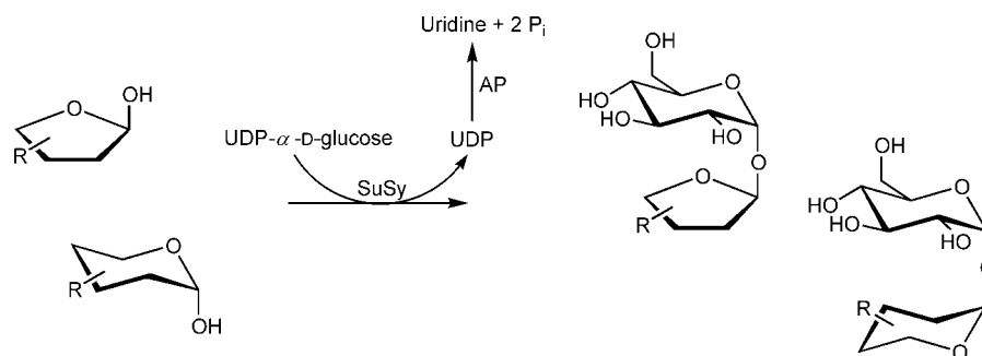
Scheme 1. General scheme for the synthesis of sucrose analogues with recombinant sucrose synthase 1 from potato.
