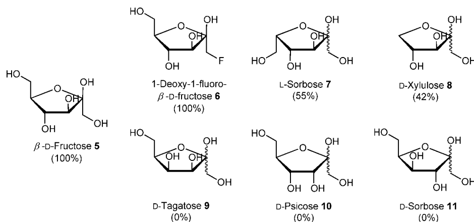
Figure 1. Ketoses as acceptor substrates for recombinant SuSy1 from potato. The monosaccharides (10 mM) were tested with the donor UDP-Glc (2 mM) in 50 mM HEPES buffer, pH 8.0, for 16 h at 30 °C. The formation of disaccharides and the conversion of UDP-Glc was monitored by HPLC. The relative yields refer to the donor substrate UDP-Glc.
